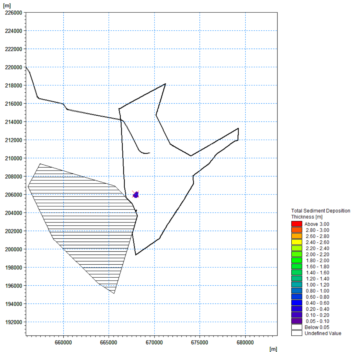
Figure 7.1157.7-409 Total deposition thickness during sediment disposal - Slack water near high-low water during neap tide ('Zone 1 & 3' material)
