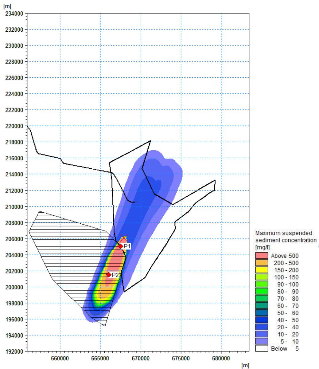
Figure 7.1167.7-66 Maximum suspended sediment concentration during array disposal occurring near the seabed – Peak flood during spring tide ('Zone 1 & 3' material) (red point = time series extraction point)
