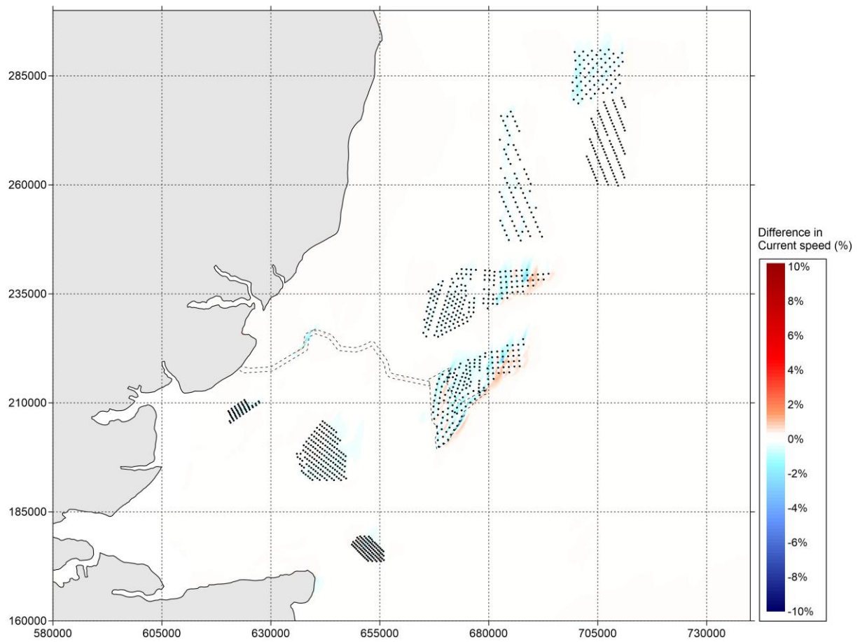
Figure 5.805.5-75 Difference in current speed (in percent) between 'Baseline' and 'Cumulative' during neap tide (positive means increase of current speed by option and vice versa) – peak ebb
