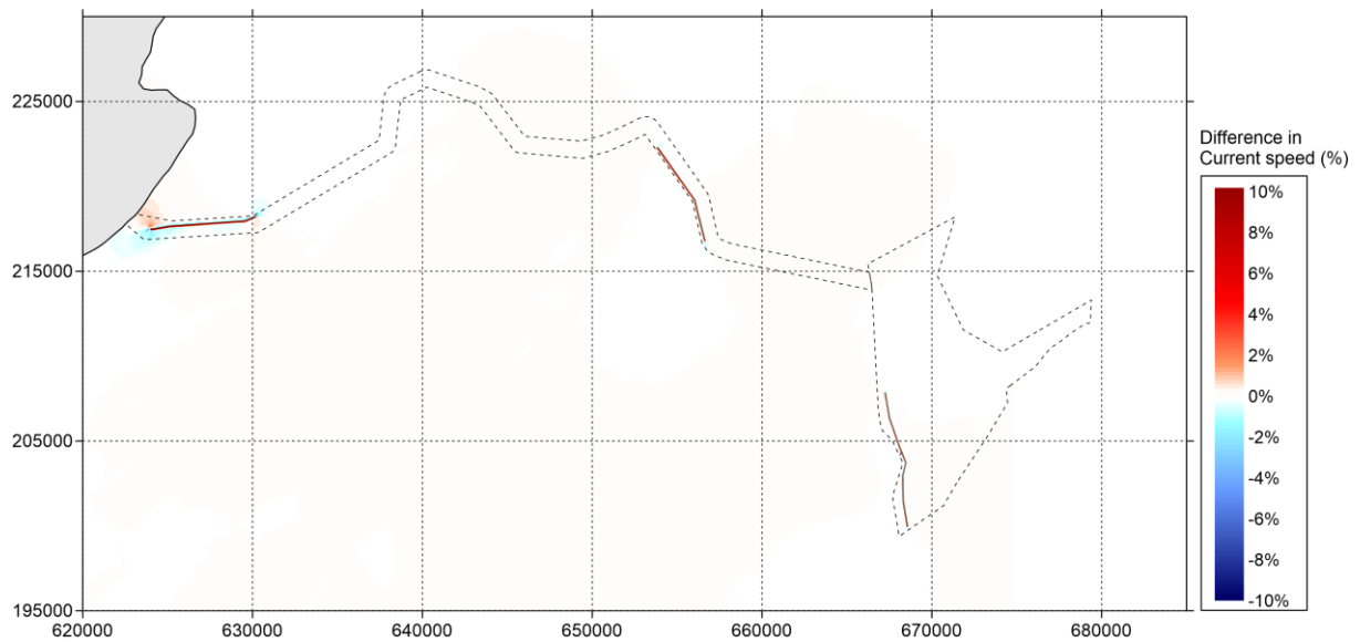
Figure 5.955.9175 Difference in current speed (in percent) between 'Baseline' and 'Additional Layout' during neap tide (positive means increase of current speed by option and vice versa) – peak flood
