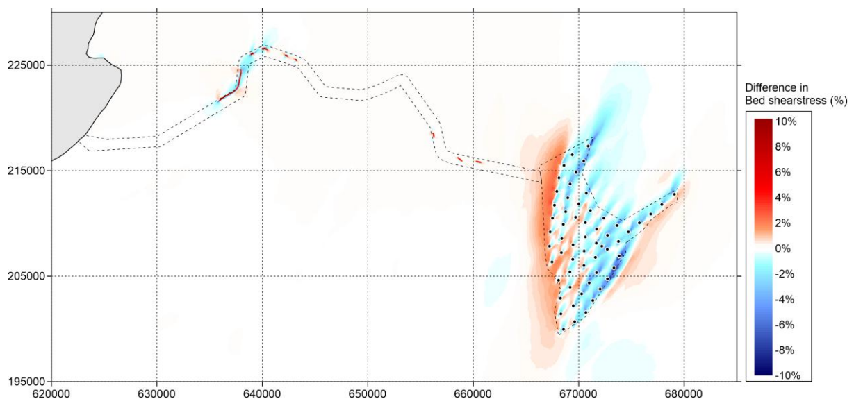
Figure 5.685.5-63 Difference in bed shear stress (in percent) between 'Baseline' and 'Option' during spring tide (positive means increase of bed shear stress by option and vice versa) – peak ebb
