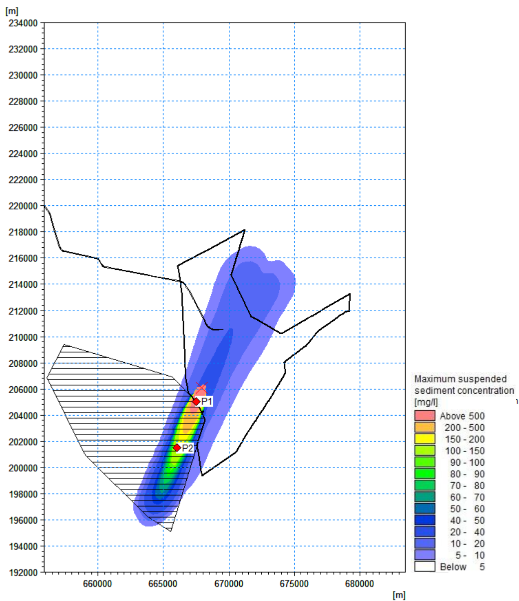
Figure 7.1187.7-68 Maximum suspended sediment concentration during array disposal occurring near the water surface – Peak flood during spring tide ('Zone 1 & 3' material) (red point = time series extraction point)
