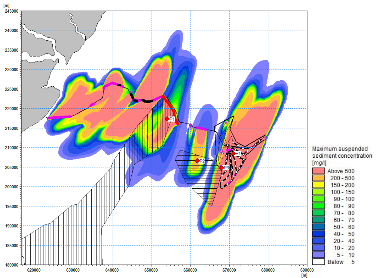
Figure 7.1347-7-428 Maximum suspended sediment concentration during an indicative offshore export cable levelling (including additional length), array cable levelling and seabed preparation operations for smaller WTGs layout structures occurring near the seabed (thick purple line = MR, thick black line = SW, white points = WTG structures , red points = time series extraction points, vertical hashed area = MLS SAC, horizontal hashed area = KKE MCZ)
