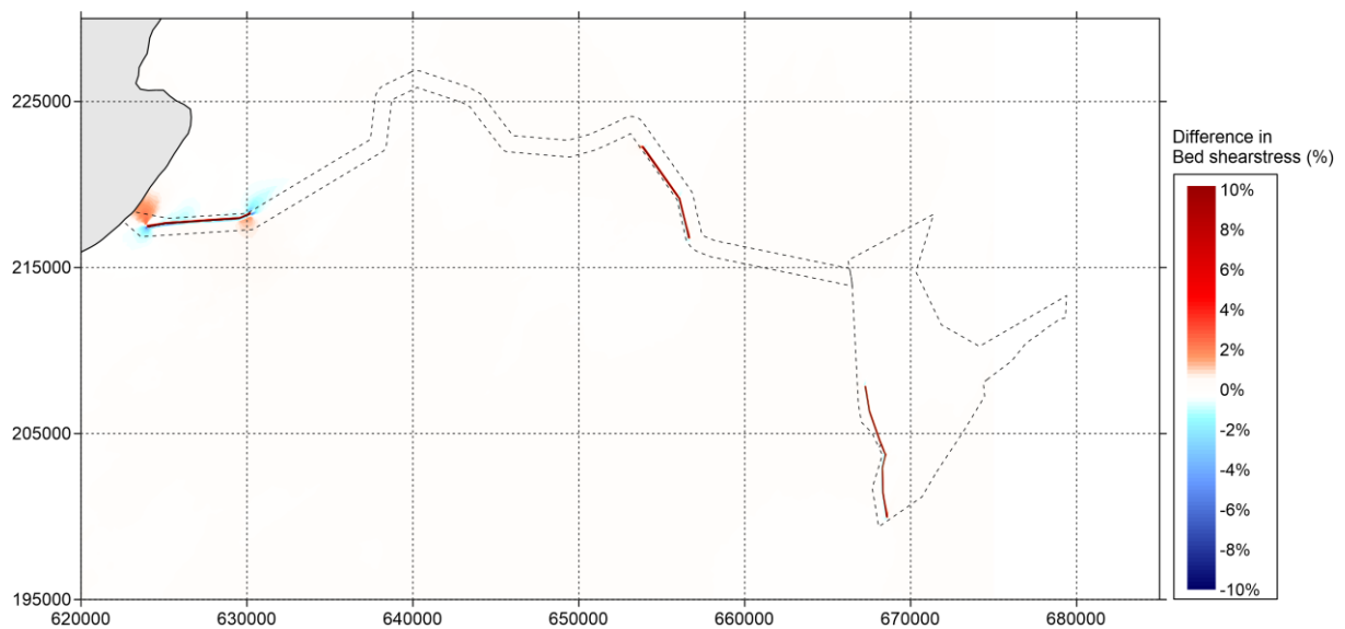
Figure 5.1045-10084 Difference in bed shear stress (in percent) between 'Baseline' and 'Additional Layout' during neap tide (positive means increase of bed shear stress by option and vice versa) – peak ebb.
