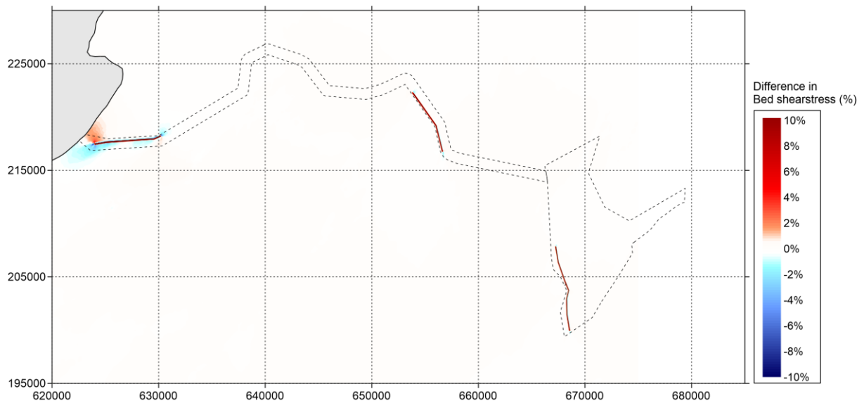
Figure 5.995.9579 Difference in bed shear stress (in percent) between 'Baseline' and 'Additional Layout' during spring tide (positive means increase of bed shear stress by option and vice versa) – peak flood
