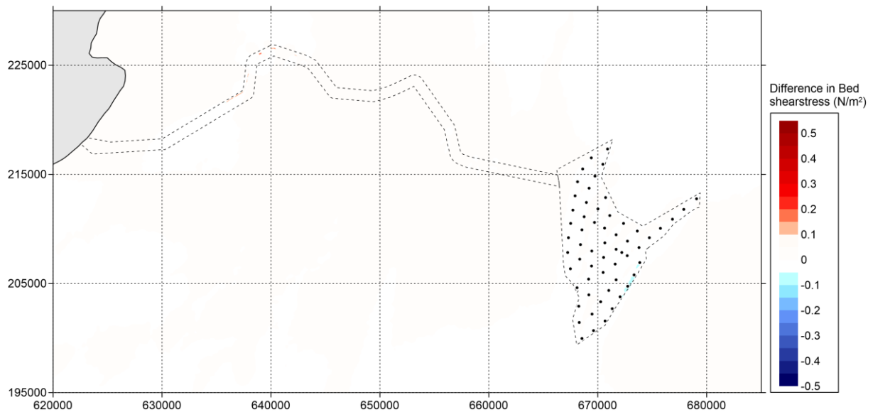
Figure 5.695.5-64 Difference in bed shear stress (in \text{N/m}^2 ) between 'Baseline' and 'Option' during neap tide (positive means increase of bed shear stress by option and vice versa) – peak flood
