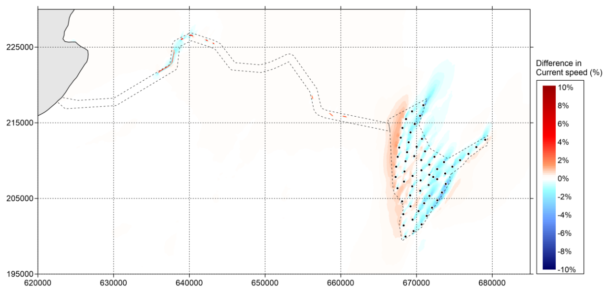
Figure 5.605-5-55 Difference in current speed (in percent) between 'Baseline' and 'Option' during spring tide (positive means increase of current speed by option and vice versa) – peak ebb
