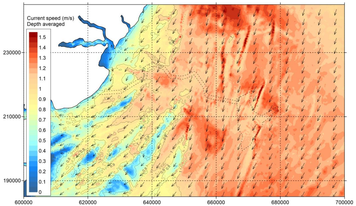
Figure 5.215.5-20 Baseline - Current speed during spring tide - peak flood (zoomed in)
