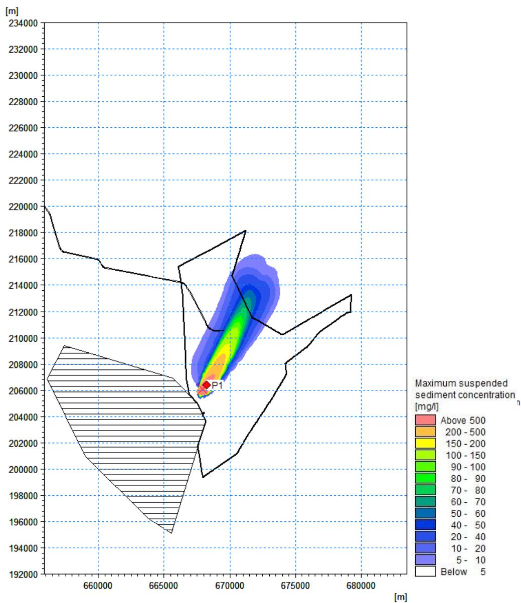
Figure 7.1077.7-105 Maximum suspended sediment concentration during array disposal occurring near the water surface – Slack water near high water during neap tide ('Zone 1 & 3' material) (red point = time series extraction point)
