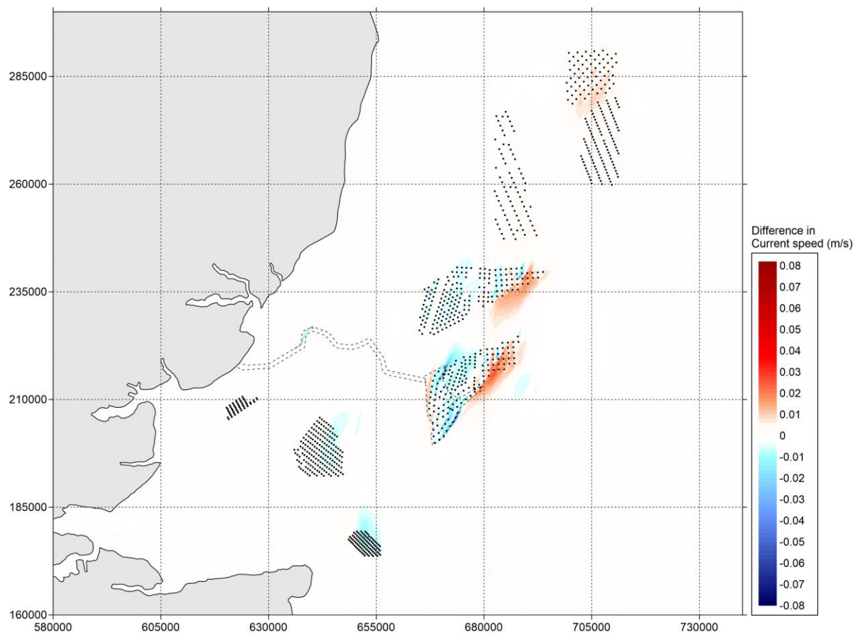
Figure 5.745.5-69 Difference in current speed (in metres/second) between 'Baseline' and 'Cumulative' during spring tide (positive means increase of current speed by option and vice versa) – peak ebb
