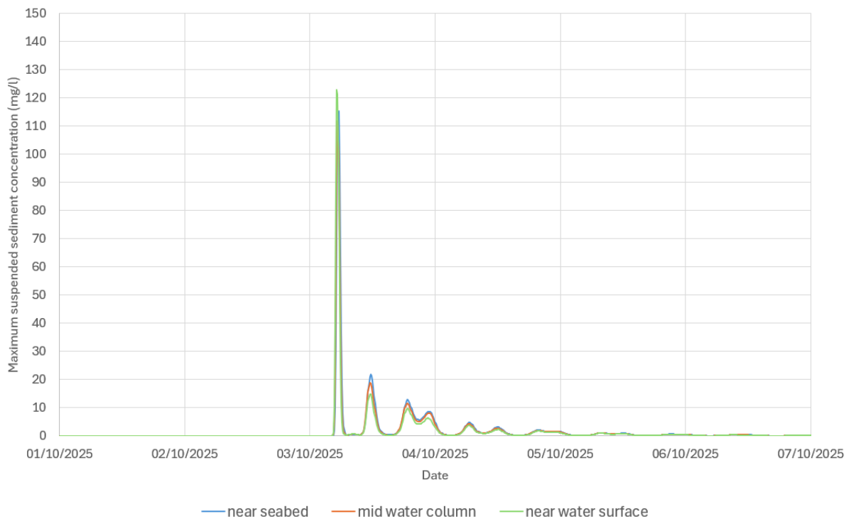
Figure 7.1147- Time series of suspended sediment concentration at P2 during sediment disposal near seabed, middle of water column and near water surface - Slack water near low water during neap tide ('Zone 1 & 3' material)
