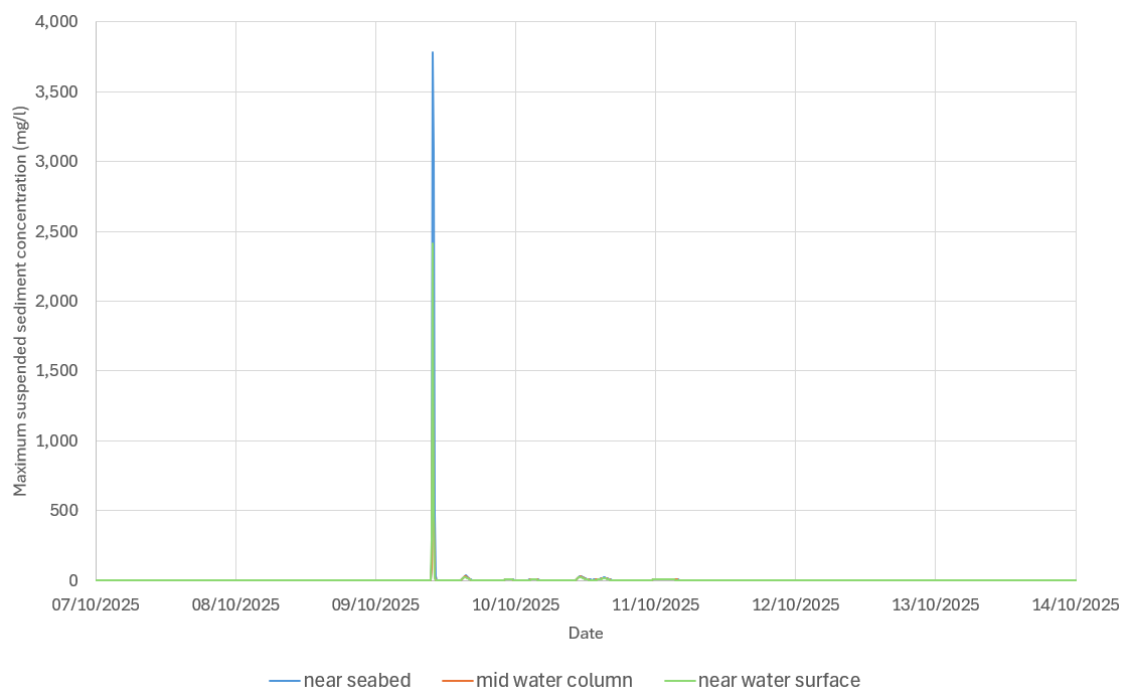
Figure 7.1197-7-119 Time series of suspended sediment concentration at P1 during sediment disposal near seabed, middle of water column and near water surface – Peak flood during spring tide ('Zone 1 & 3' material)
