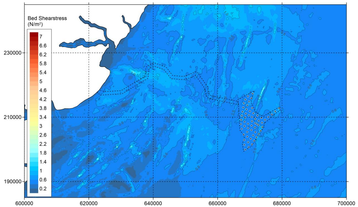
Figure 5.475-5-46 Option – Bed shear stress during neap tide - peak flood.
