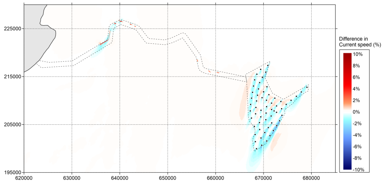
Figure 5.595-5-54 Difference in current speed (in percent) between 'Baseline' and 'Option' during spring tide (positive means increase of current speed by option and vice versa) – peak flood
