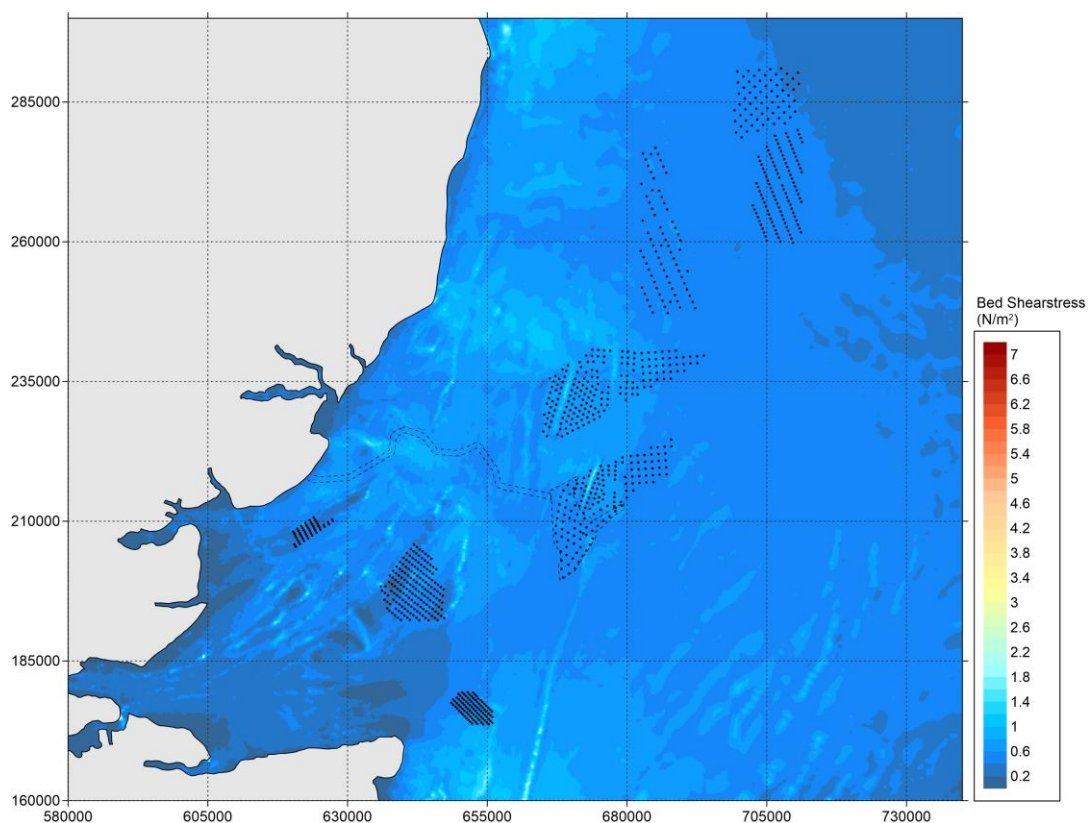
Figure 5.515-5-50 All windfarms ('Cumulative') – Bed shear stress during neap tide – peak flood.
