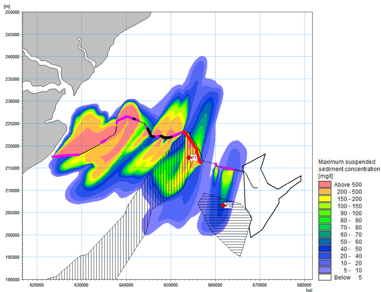
Figure 7.1297: Maximum suspended sediment concentration during an indicative offshore export cable levelling (including additional length) in the middle of water column (thick purple line = MR, thick black line = SW, red points = time series extraction points, vertical hashed area = MLS SAC, horizontal hashed area = KKE MCZ)
