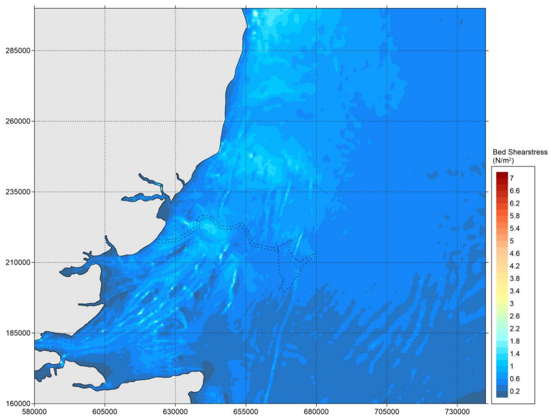
Figure 5.445-5-43 Baseline – Bed shear stress during neap tide - peak ebb (zoomed out).
