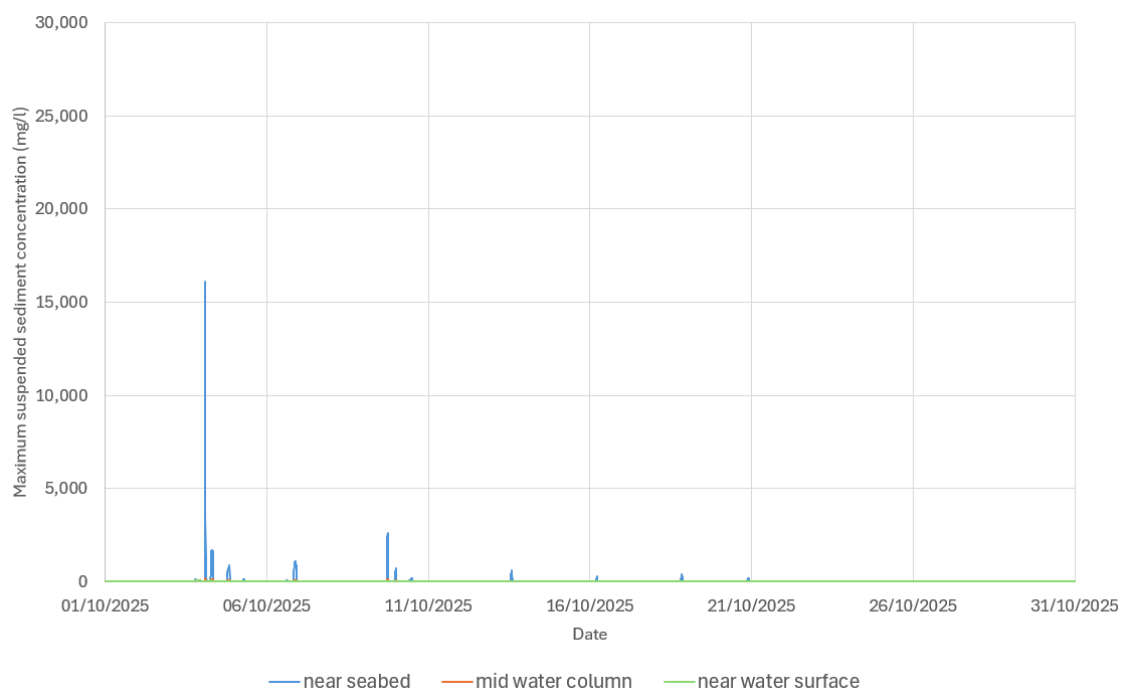
Figure 7.1397: Time series of suspended sediment concentration at P3 during indicative offshore export cable levelling (including additional length), array cable levelling and seabed preparation operations for smaller WTGs layout structures for seabed, middle of water column and near water surface (near KKE MCZ)
