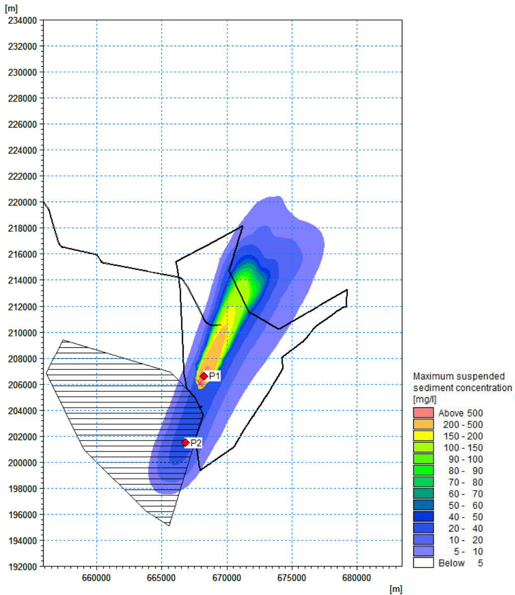
Figure 7.1237.7-417 Maximum suspended sediment concentration during array disposal occurring near the middle of water column – Peak flood ebb during spring tide ('Zone 1 & 3' material) (red point = time series extraction point)
