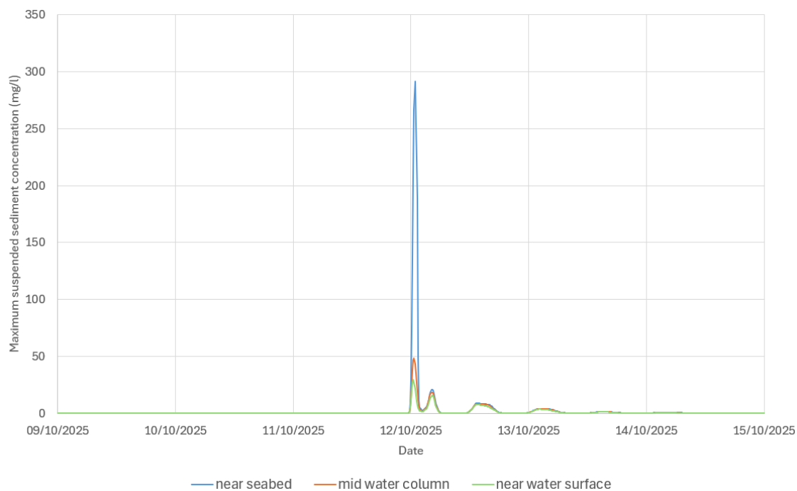
Figure 7.1327-7-434 Time series of suspended sediment concentration at P1 during indicative offshore export cable levelling (including additional length) for seabed, middle of water column and near water surface (inside MSL SACKKE MCZ )
