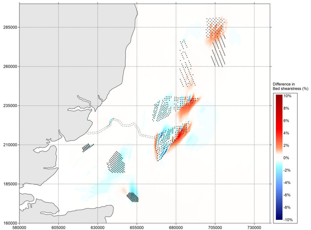
Figure 5.845.5-79 Difference in bed shear stress (in percent) between 'Baseline' and 'Cumulative' during spring tide (positive means increase of bed shear stress by option and vice versa) – peak ebb.
