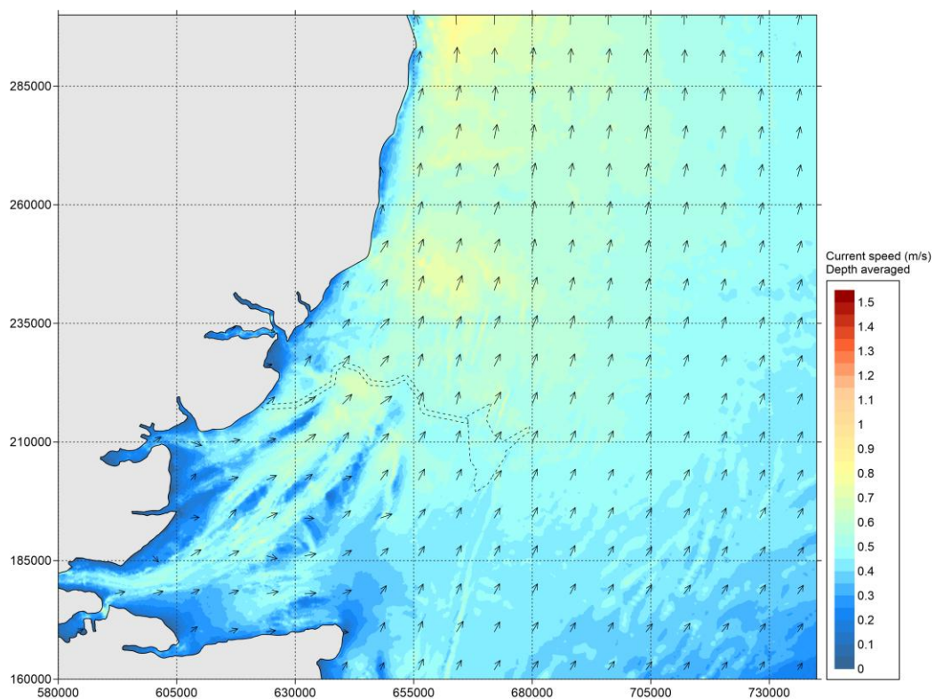
Figure 5.285-5-27 Baseline - Current speed during neap tide - peak ebb (zoomed out).
