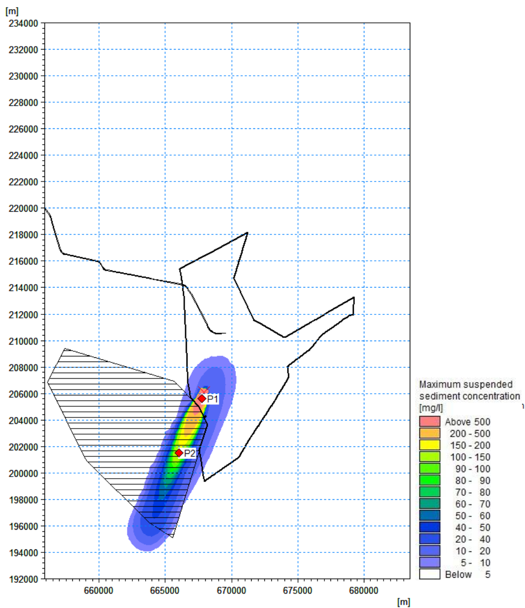
Figure 7.1127.7-107 Maximum suspended sediment concentration during array disposal occurring near the water surface – Slack water near high-low water during neap tide ('Zone 1 & 3' material) (red point = time series extraction point)
