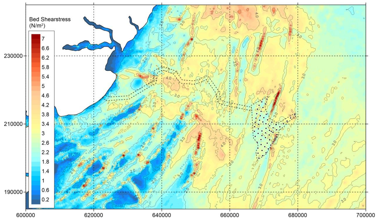
Figure 5.455-5-44 Option – Bed shear stress during spring tide - peak flood.
