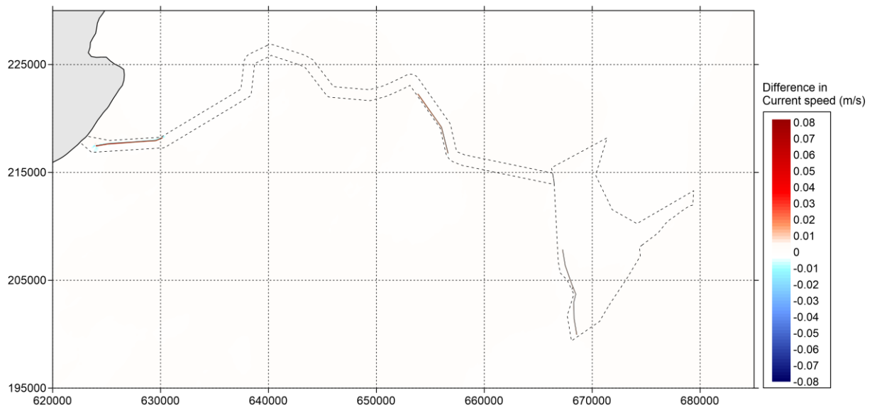
Figure 5.935-8973 Difference in current speed (in metres/second) between 'Baseline' and 'Additional Layout' during neap tide (positive means increase of current speed by option and vice versa) – peak flood
