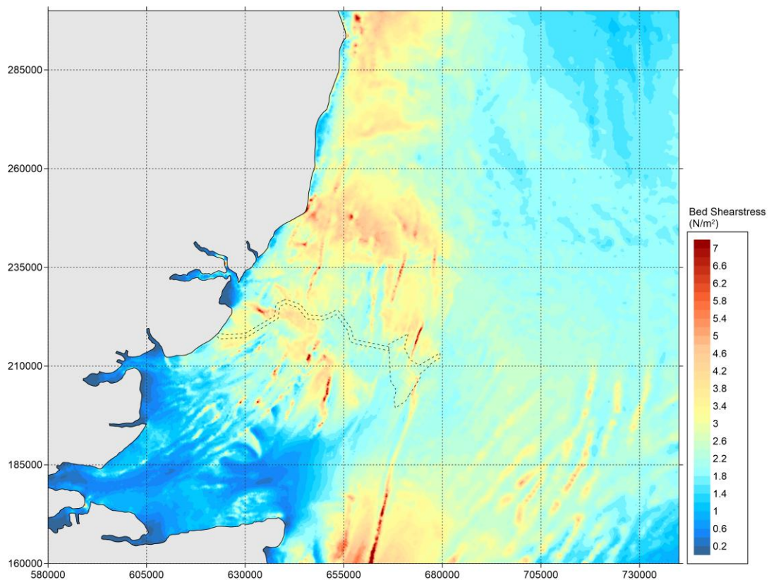
Figure 5.405.5-39 Baseline – Bed shear stress during spring tide - peak ebb (zoomed out).
