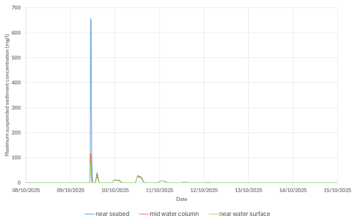
Figure 7.1267.7-120 Time series of suspended sediment concentration at P2 during sediment disposal near seabed, middle of water column and near water surface – Peak flood ebb during spring tide ('Zone 1 & 3' material)
