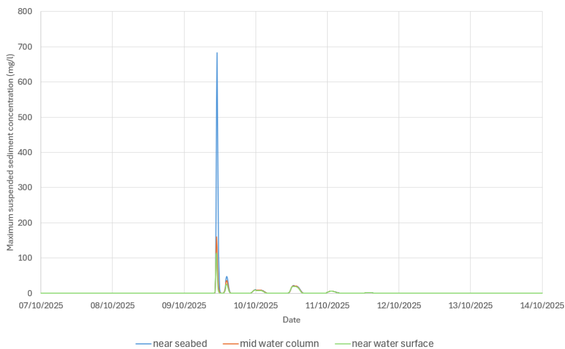
Figure 7.1207-7-120 Time series of suspended sediment concentration at P2 during sediment disposal near seabed, middle of water column and near water surface – Peak flood during spring tide ('Zone 1 & 3' material)
