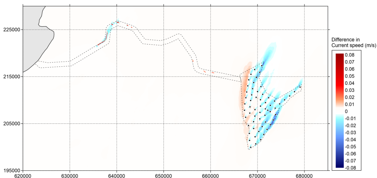
Figure 5.575-5-52 Difference in current speed (in metres/second) between 'Baseline' and 'Option' during spring tide (positive means increase of current speed by option and vice versa) – peak flood
