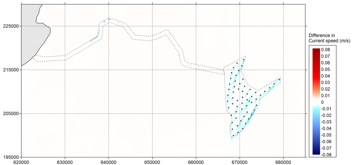
Figure 5.615.5-56 Difference in current speed (in metres/second) between 'Baseline' and 'Option' during neap tide (positive means increase of current speed by option and vice versa) – peak flood
