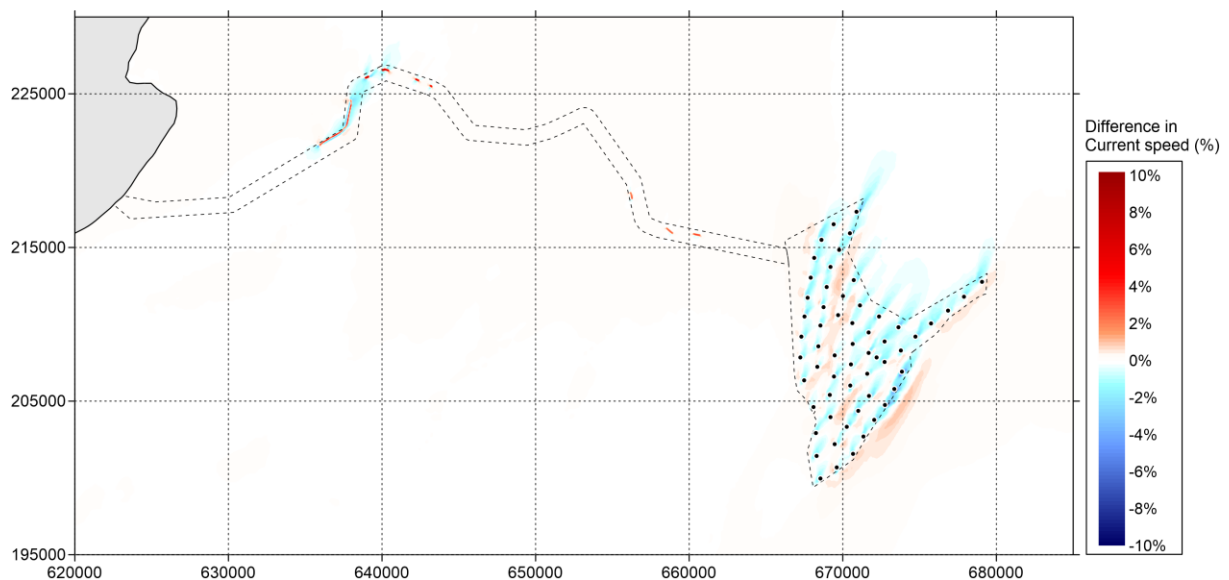
Figure 5.645-5-59 Difference in current speed (in percent) between 'Baseline' and 'Option' during neap tide (positive means increase of current speed by option and vice versa) – peak ebb
