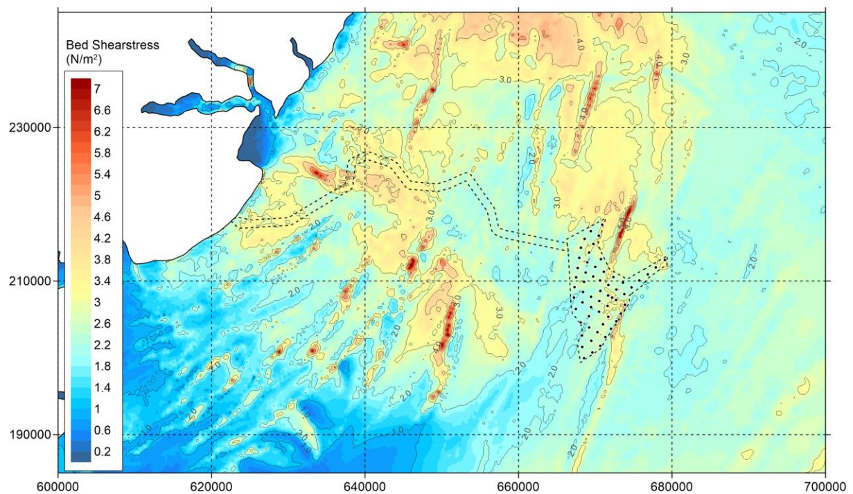
Figure 5.465-5-45 Option – Bed shear stress during spring tide - peak ebb.
