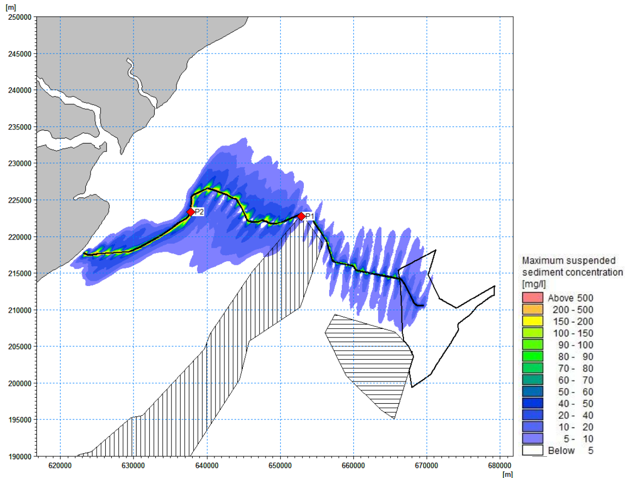
Figure 7.7 Maximum suspended sediment concentration during offshore export cable trenching operations occurring near the seabed (red points = time series extraction points, vertical hashed area = MLS SAC, horizontal hashed area = KKE MCZ)
