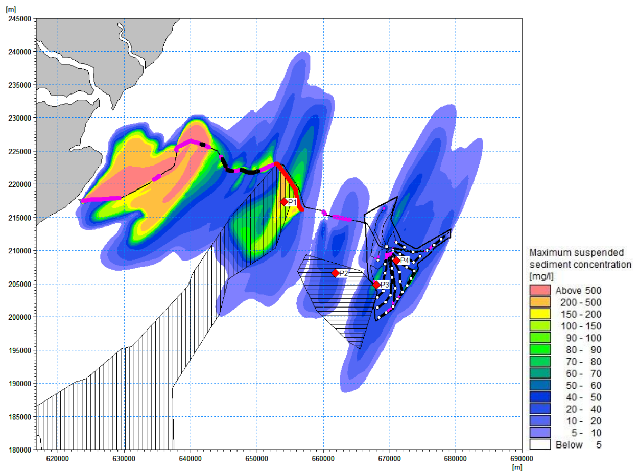
Figure 7.1367-7-434 Maximum suspended sediment concentration during an indicative offshore export cable levelling (including additional length), array cable levelling and seabed preparation operations for smaller WTGs layout structures occurring occurring near the seabed water surface (thick purple line = MR, thick black line = SW, white points = WTG structures, red points = time series extraction points, vertical hashed area = MLS SAC, horizontal hashed area = KKE MCZ)
