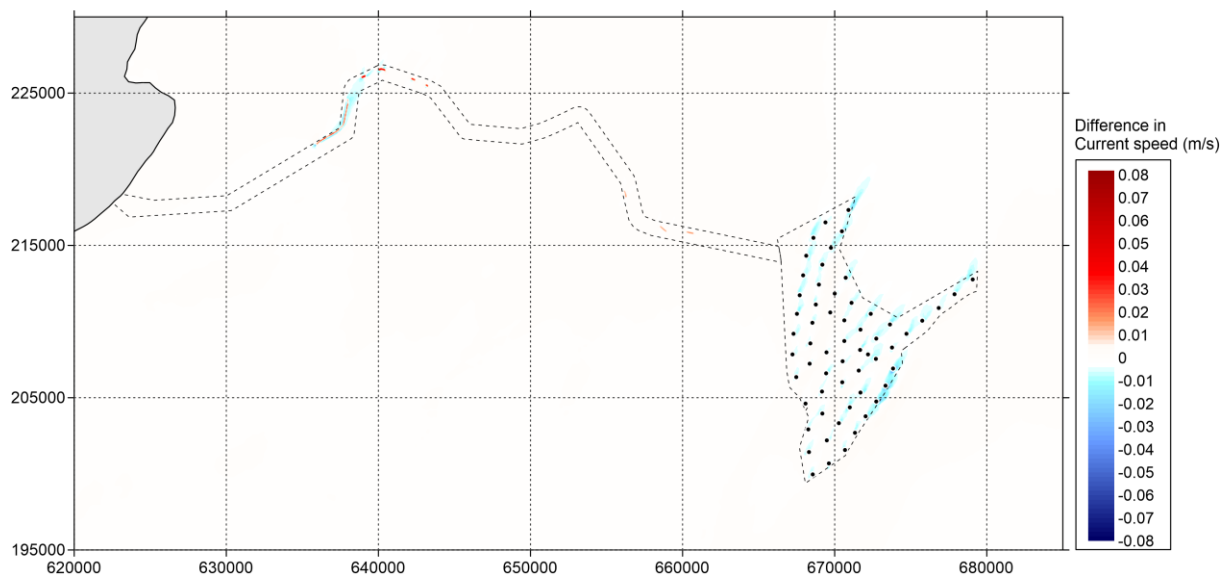
Figure 5.625.5-57 Difference in current speed (in metres/second) between 'Baseline' and 'Option' during neap tide (positive means increase of current speed by option and vice versa) – peak ebb
