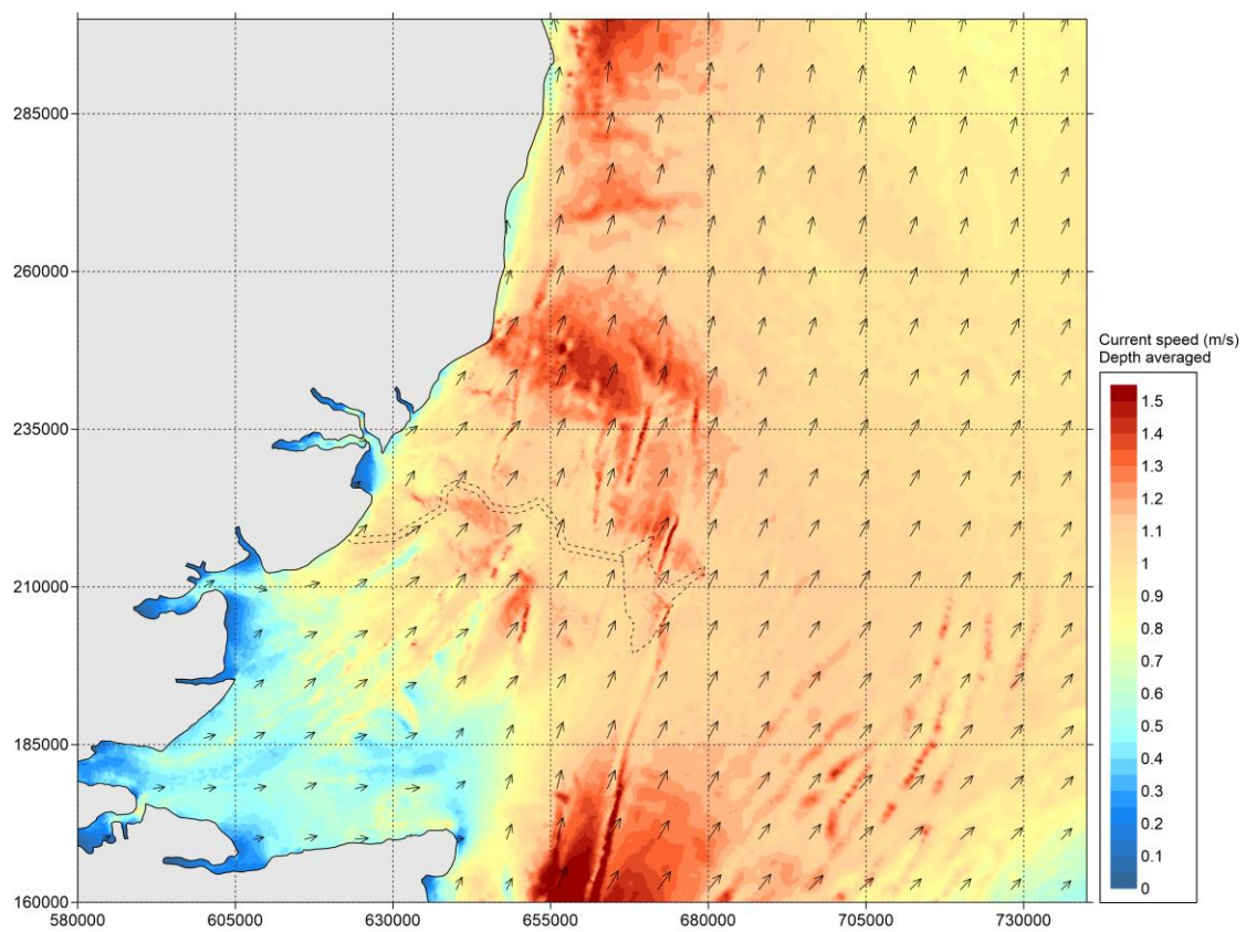
Figure 5.245-5-23 Baseline - Current speed during spring tide - peak ebb (zoomed out)
