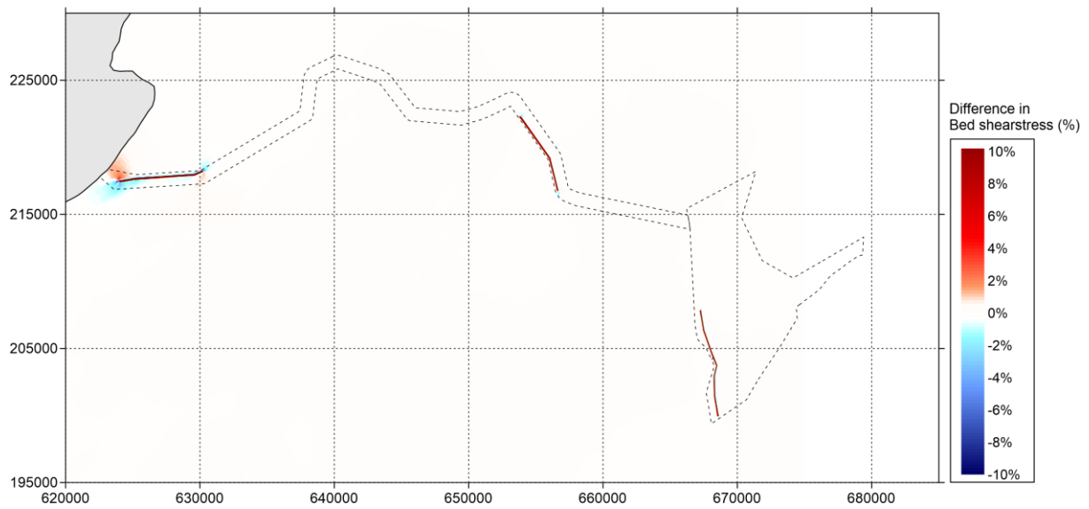
Figure 5.1035-9983 Difference in bed shear stress (in percent) between 'Baseline' and 'Additional Layout' during neap tide (positive means increase of bed shear stress by option and vice versa) – peak flood.
