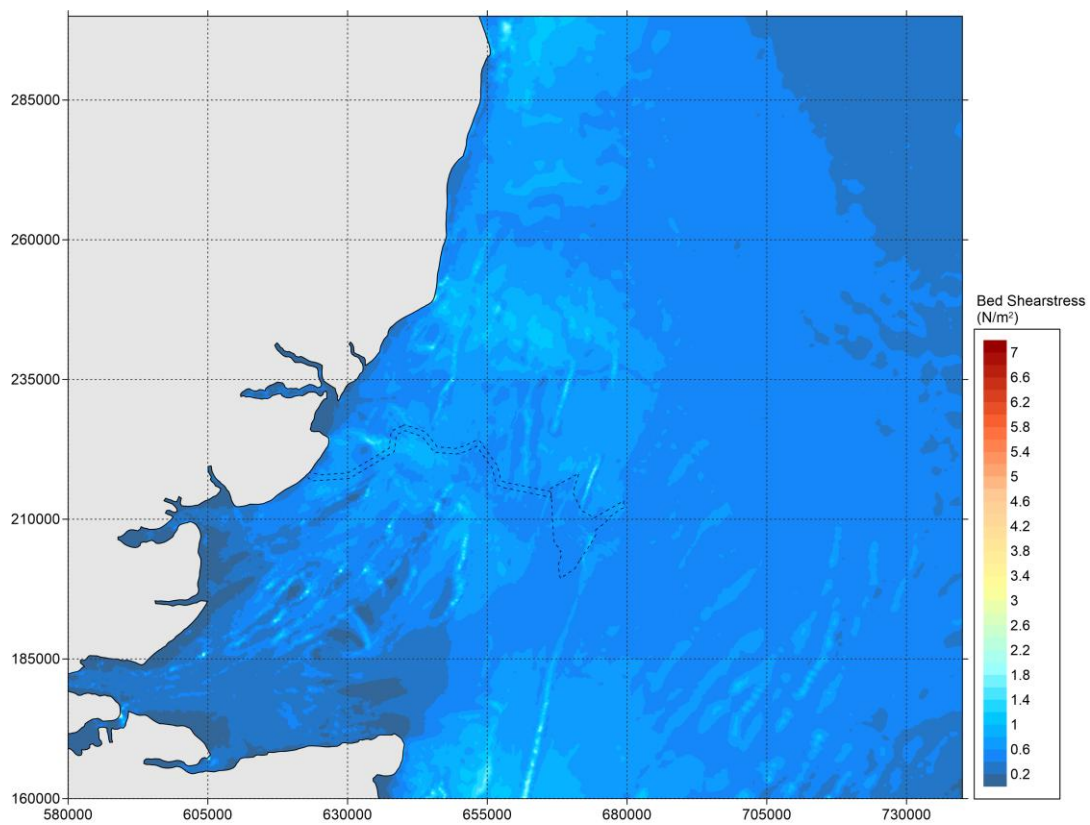
Figure 5.425.5-41 Baseline – Bed shear stress during neap tide - peak flood (zoomed out)
