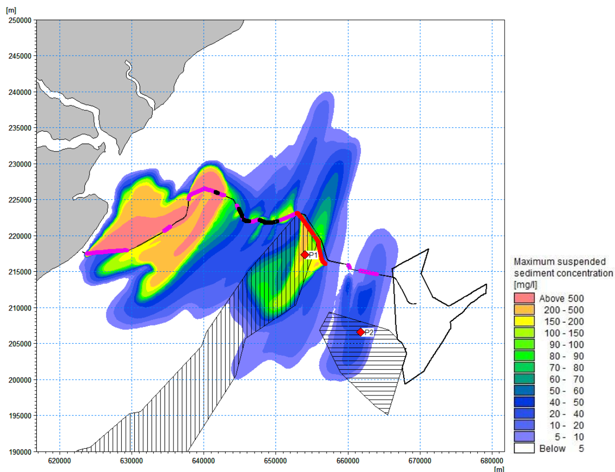
Figure 7.1307- Maximum suspended sediment concentration during an indicative offshore export cable levelling (including additional length) near the water surface (thick purple line = MR, thick black line = SW, red points = time series extraction points, vertical hashed area = MLS SAC, horizontal hashed area = KKE MCZ)
