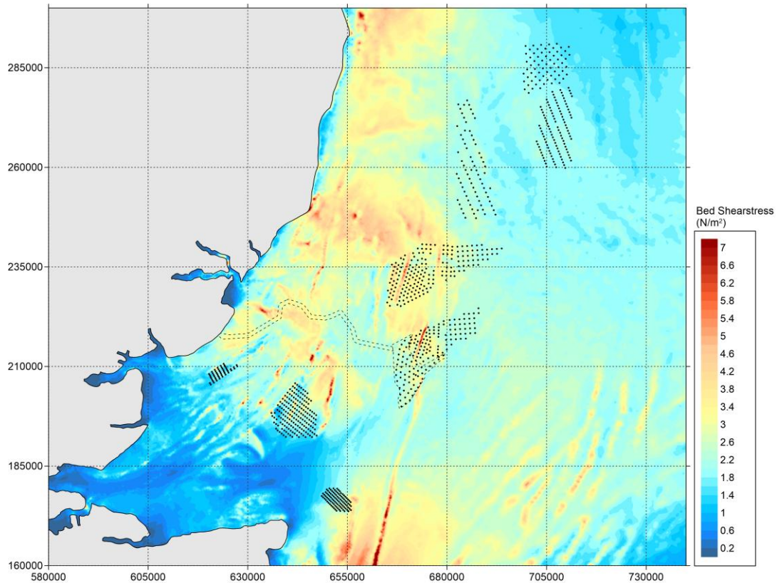
Figure 5.495.5-48 All windfarms ('Cumulative') – Bed shear stress during spring tide - peak flood.
