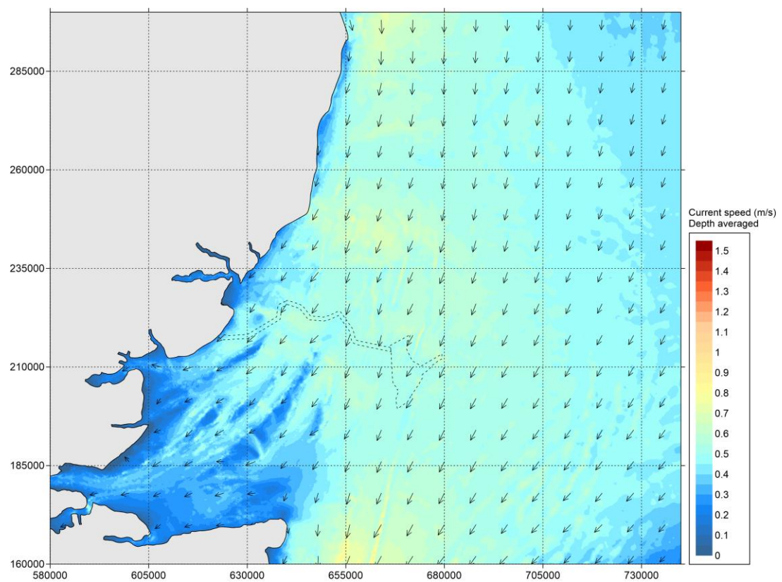
Figure 5.265-5-25 Baseline - Current speed during neap tide - peak flood (zoomed out).
