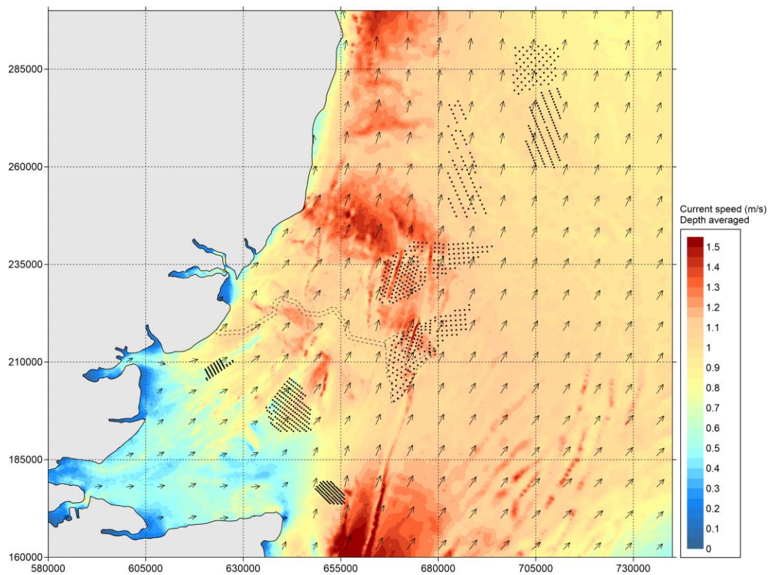
Figure 5.345-5-33 All windfarms ('Cumulative') - Current speed during spring tide - peak ebb.
