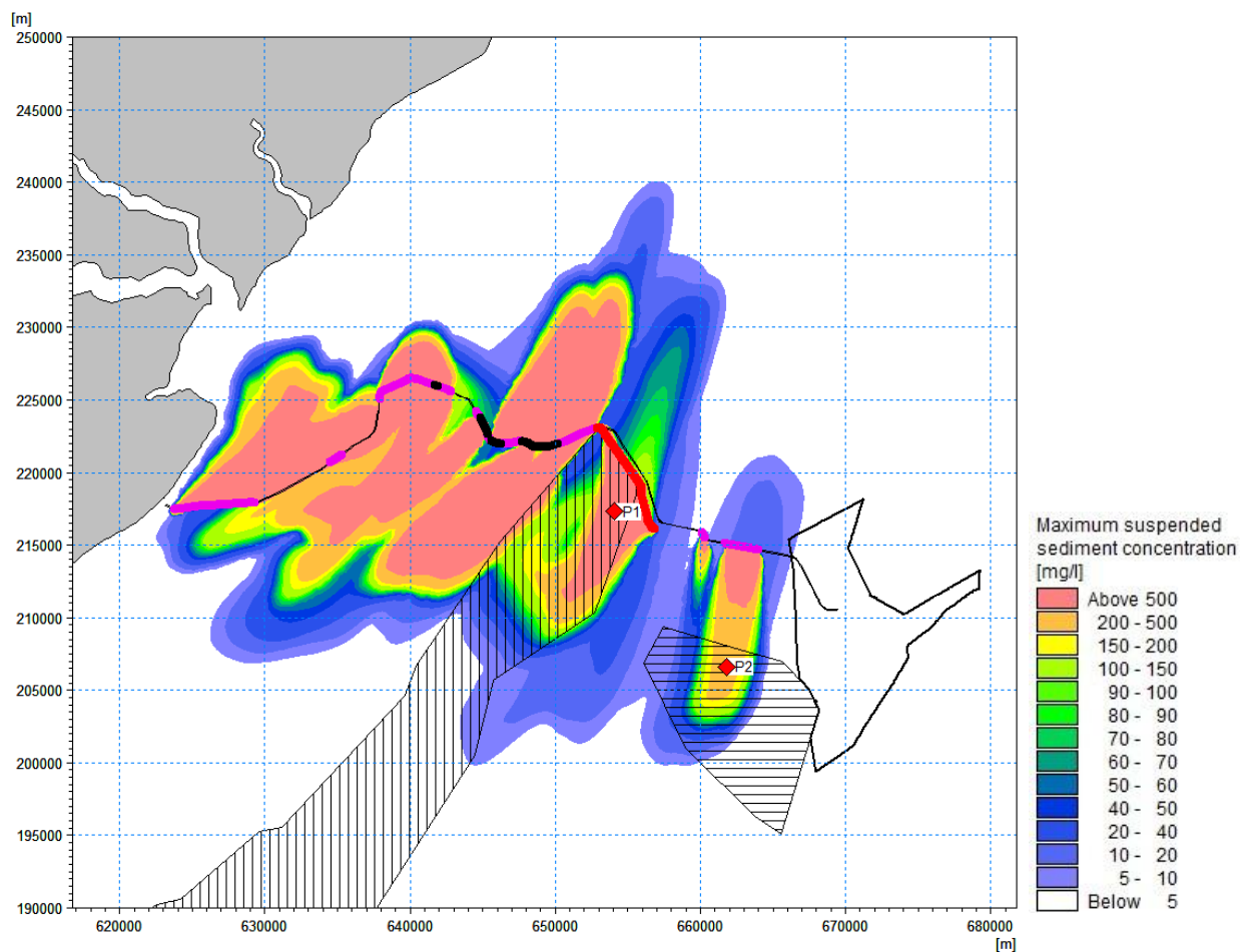
Figure 7.1287.7-4 Maximum suspended sediment concentration during an indicative offshore export cable levelling (including additional length) near the seabed (thick purple line = MR, thick black line = SW, red points = time series extraction points, vertical hashed area = MLS SAC, horizontal hashed area = KKE MCZ)
