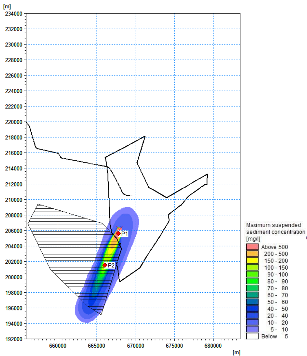
Figure 7.1117.7-106 Maximum suspended sediment concentration during array disposal occurring near middle of water column– Slack water near high-low water during neap tide ('Zone 1 & 3' material) (red point = time series extraction point)
