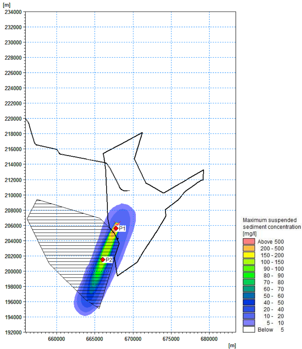
Figure 7.1107.7-105 Maximum suspended sediment concentration during array disposal occurring near the seabed – Slack water near high-low water during neap tide ('Zone 1 & 3' material) (red point = time series extraction point)
