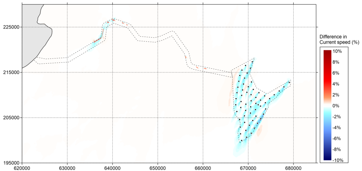
Figure 5.635-5-58 Difference in current speed (in percent) between 'Baseline' and 'Option' during neap tide (positive means increase of current speed by option and vice versa) – peak flood
