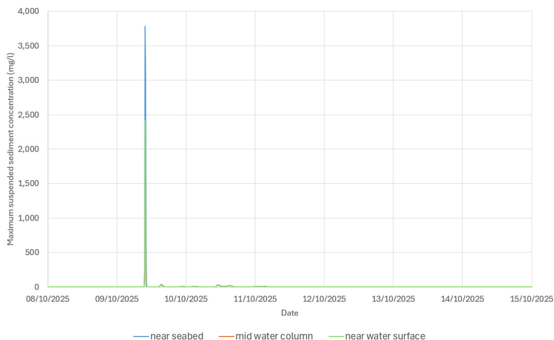
Figure 7.1257.7-119 Time series of suspended sediment concentration at P1 during sediment disposal near seabed, middle of water column and near water surface – Peak flood ebb during spring tide ('Zone 1 & 3' material)
