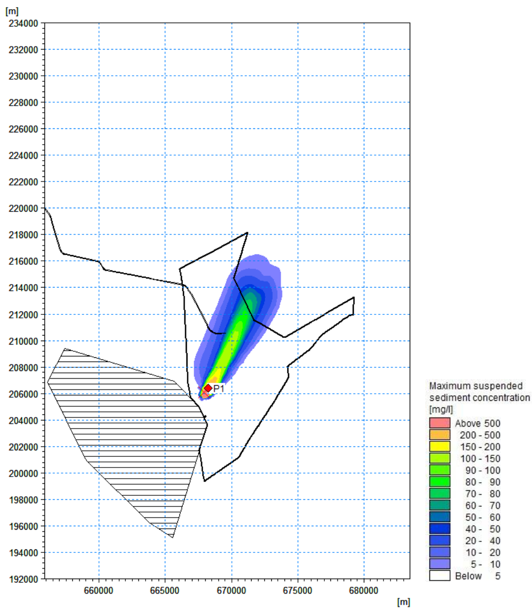
Figure 7.1057.7-55 Maximum suspended sediment concentration during array disposal occurring near the seabed – Slack water near high water during neap tide ('Zone 1 & 3' material) (red point = time series extraction point)
