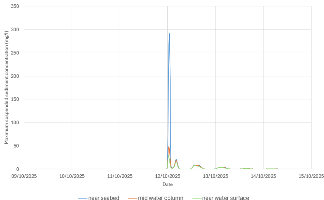
Figure 7.138- Time series of suspended sediment concentration at P2 during indicative offshore export cable levelling (including additional length), array cable levelling and seabed preparation operations for smaller WTGs layout structures for seabed, middle of water column and near water surface (inside KKE MCZ)
