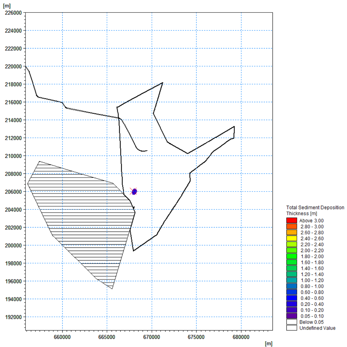
Figure 7.1097.7-59 Total deposition thickness during sediment disposal - Slack water near high water during neap tide ('Zone 1 & 3' material)
