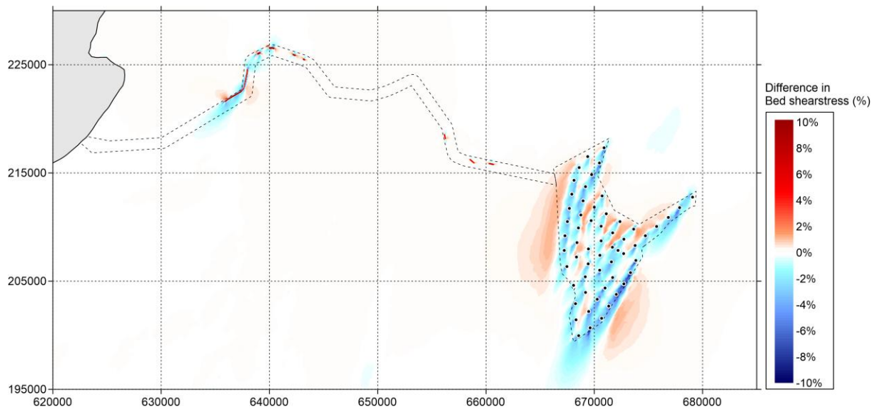
Figure 5.675.5-62 Difference in bed shear stress (in percent) between 'Baseline' and 'Option' during spring tide (positive means increase of bed shear stress by option and vice versa) – peak flood
