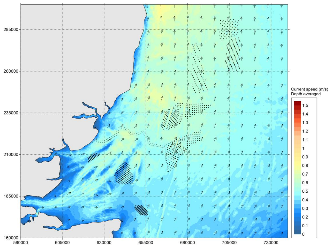
Figure 5.365-5-35 All windfarms ('Cumulative') - Current speed during neap tide - peak ebb.
