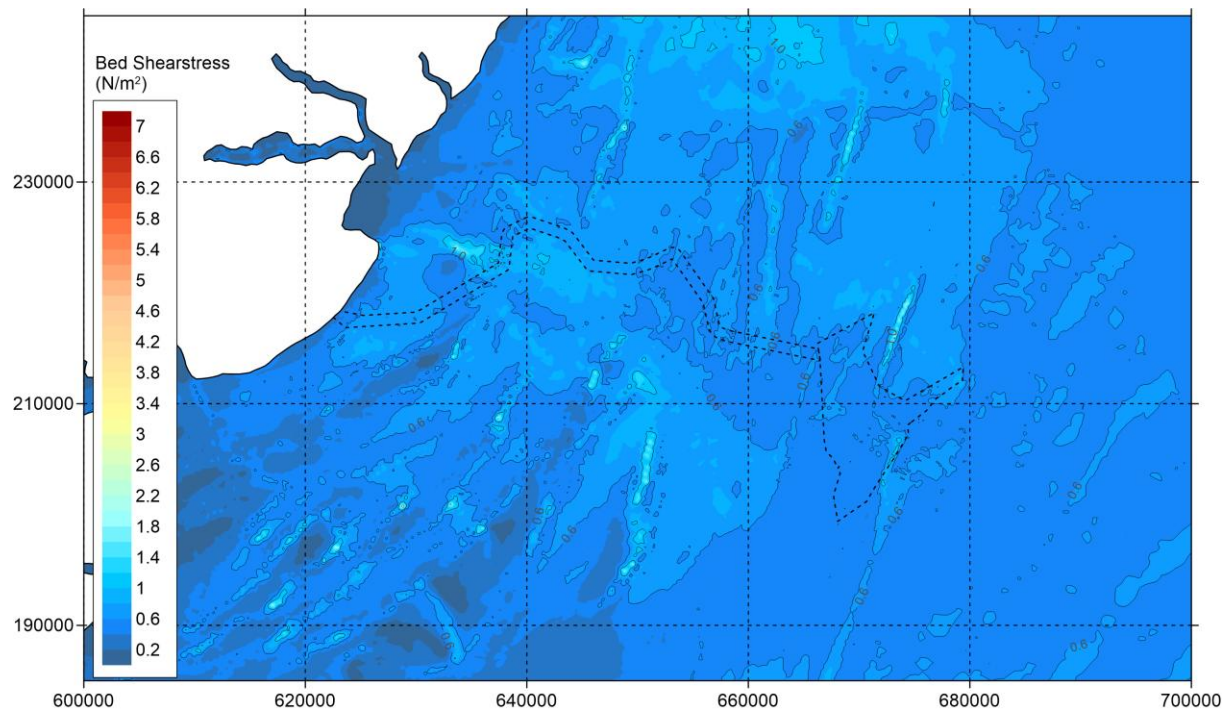
Figure 5.415.5-40 Baseline – Bed shear stress during neap tide - peak flood (zoomed in).
