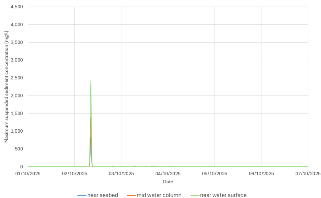
Figure 7.1087.7-58 Time series of suspended sediment concentration at P1 during sediment disposal near seabed, middle of water column and near water surface - Slack water near high water during neap tide ('Zone 1 & 3' material)
