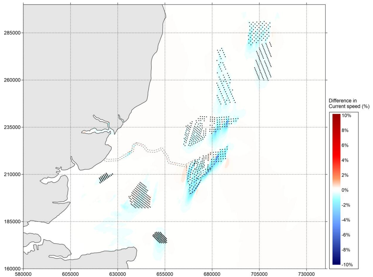
Figure 5.755-5-70 Difference in current speed (in percent) between 'Baseline' and 'Cumulative' during spring tide (positive means increase of current speed by option and vice versa) – peak flood
