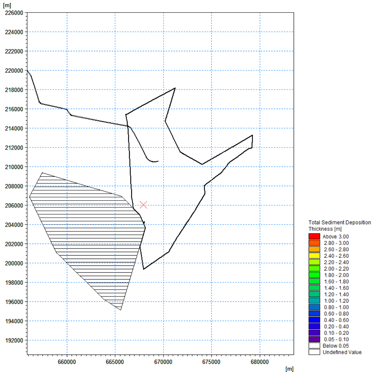
Figure 7.127-7-124 Total deposition thickness during sediment disposal - Peak flood-ebb during spring tide ('Zone 1 & 3' material)
