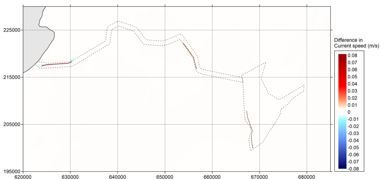
Figure 5.905.8670 Difference in current speed (in metres/second) between 'Baseline' and 'Additional Layout' during spring tide (positive means increase of current speed by option and vice versa) – peak ebb
