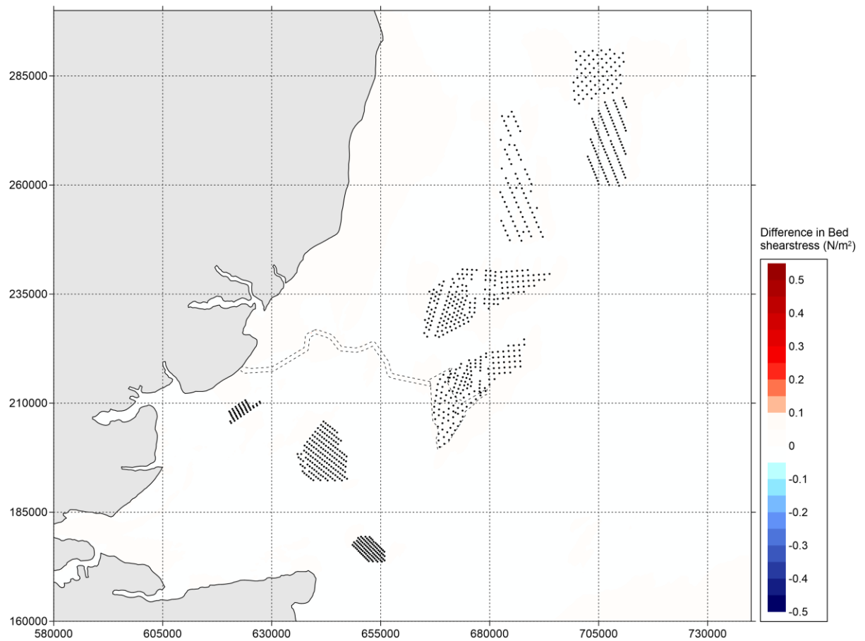
Figure 5.865.5-84 Difference in bed shear stress (in N/m 2 ) between 'Baseline' and 'Cumulative' during neap tide (positive means increase of bed shear stress by option and vice versa) – peak ebb.
