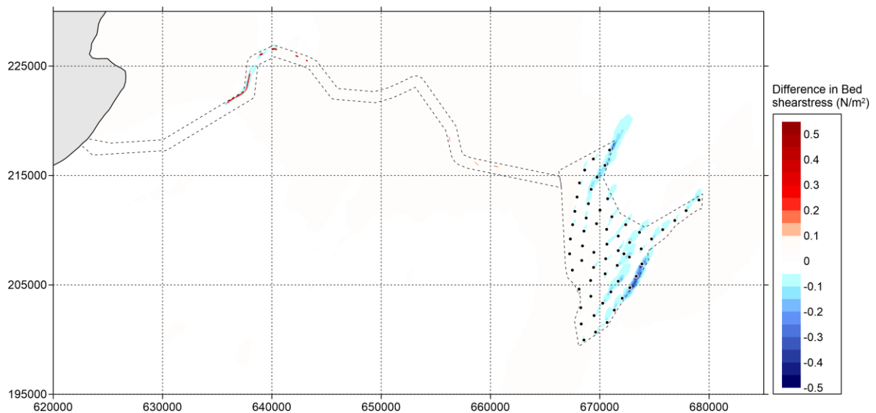
Figure 5.665-5-64 Difference in bed shear stress (in \text{N/m}^2 ) between 'Baseline' and 'Option' during spring tide (positive means increase of bed shear stress by option and vice versa) – peak ebb
