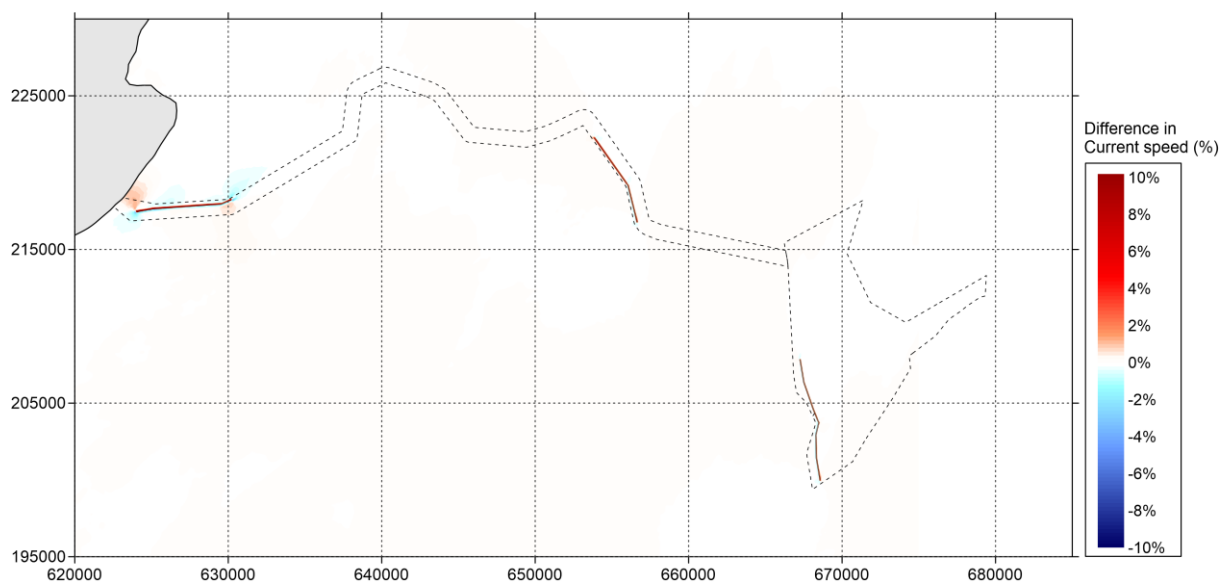
Figure 5.965.9276 Difference in current speed (in percent) between 'Baseline' and 'Additional Layout' during neap tide (positive means increase of current speed by option and vice versa) – peak ebb
