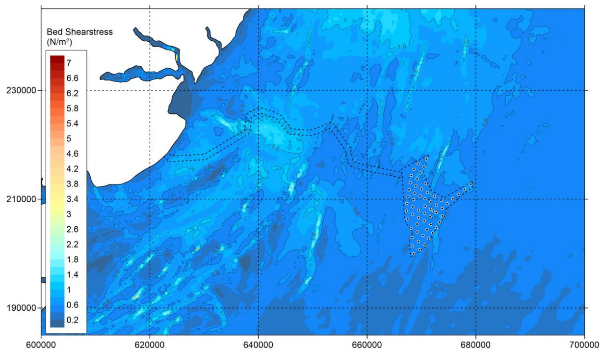
Figure 5.485-5-47 Option – Bed shear stress during neap tide - peak ebb.
