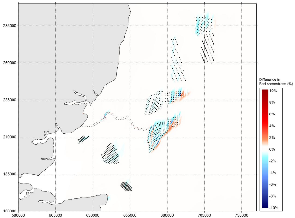
Figure 5.885.5-83 Difference in bed shear stress (in percent) between 'Baseline' and 'Cumulative' during neap tide (positive means increase of bed shear stress by option and vice versa) – peak ebb.
