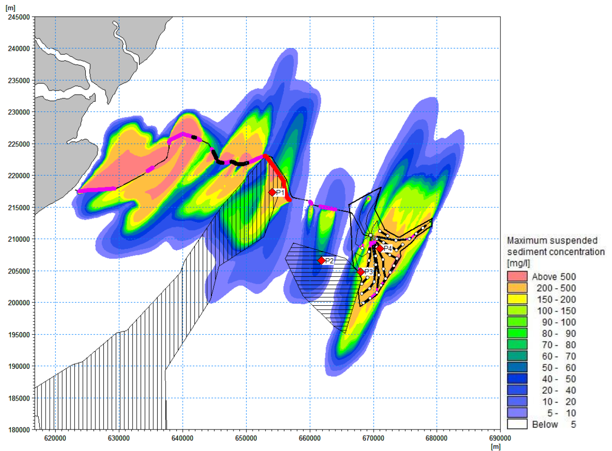
Figure 7.1357-7-434 Maximum suspended sediment concentration during an indicative offshore export cable levelling (including additional length), array cable levelling and seabed preparation operations for smaller WTGs layout structures occurring occurring near the seabed middle of water column (thick purple line = MR, thick black line = SW, white points = WTG structures, red points = time series extraction points, vertical hashed area = MLS SAC, horizontal hashed area = KKE MCZ)
