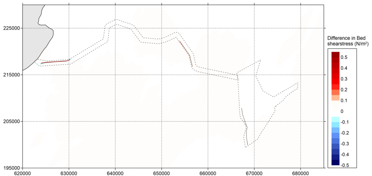
Figure 5.985.9478 Difference in bed shear stress (in \text{N/m}^2 ) between 'Baseline' and 'Additional Layout' during spring tide (positive means increase of bed shear stress by option and vice versa) – peak ebb
