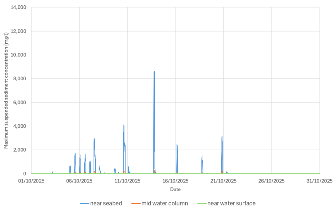
Figure 7.1407: Time series of suspended sediment concentration at P4 during indicative offshore export cable levelling (including additional length), array cable levelling and seabed preparation operations for smaller WTGs layout structures for seabed, middle of water column and near water surface (array centre)
