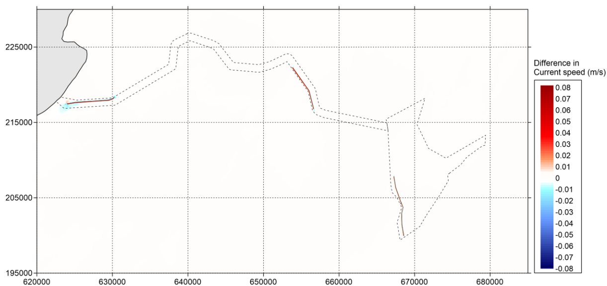
Figure 5.895.8569 Difference in current speed (in metres/second) between 'Baseline' and 'Additional Layout' during spring tide (positive means increase of current speed by option and vice versa) – peak flood
