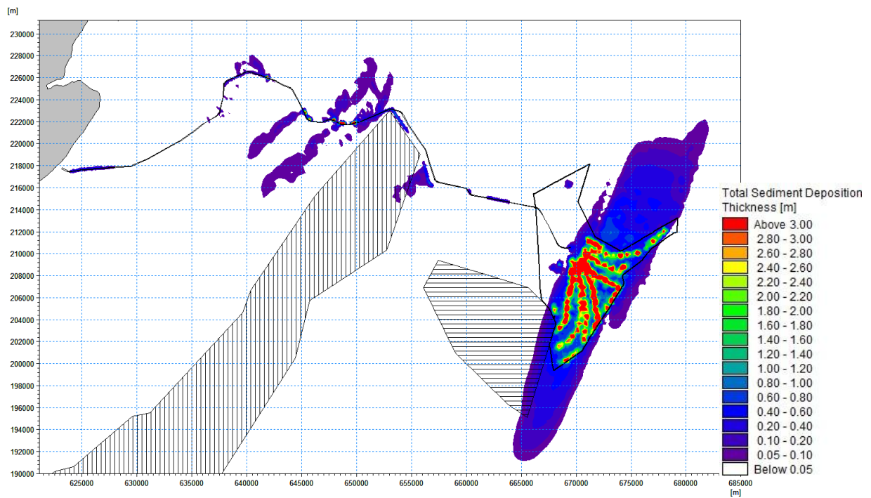
Figure 7.1417-7-436 Maximum suspended sediment concentration-Total sediment deposition thickness during an indicative offshore export cable levelling (including additional length), array cable levelling and seabed preparation operations for smaller WTGs layout structures occurring near the water surface (thick purple line = MR, thick black line = SW, white points = WTG structures, red points = time series extraction points, vertical hashed area = MLS SAC, horizontal hashed area = KKE MCZ)
