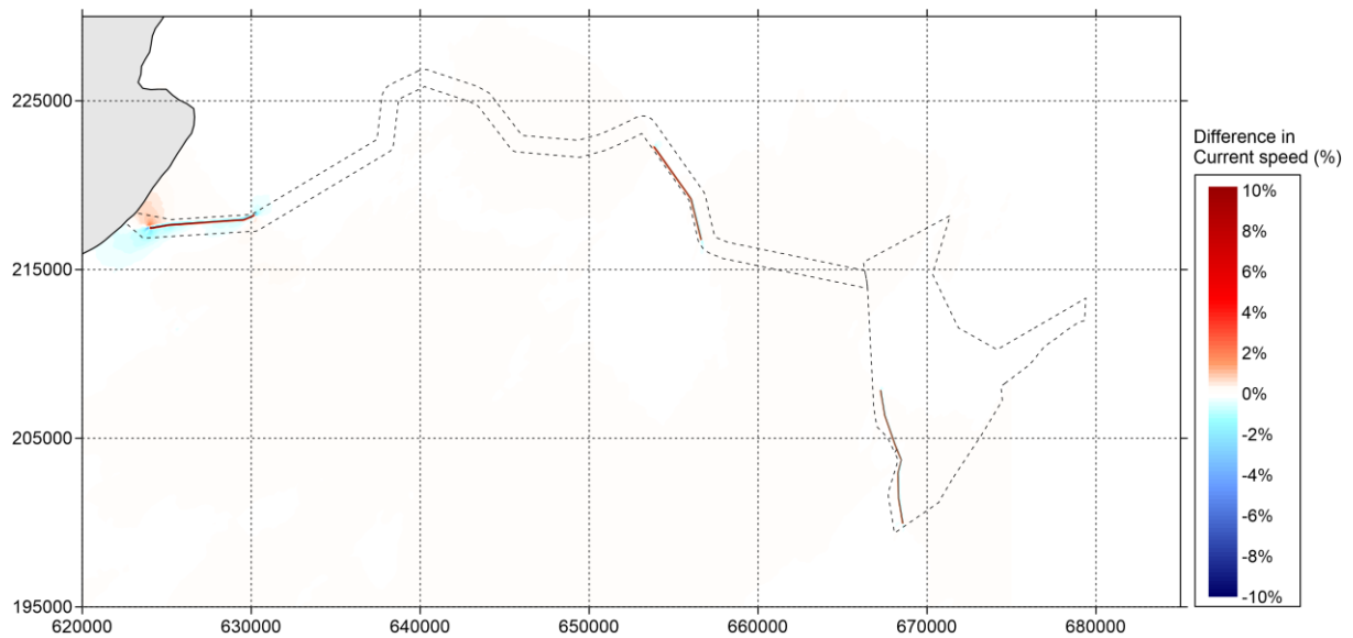
Figure 5.915.8774 Difference in current speed (in percent) between 'Baseline' and 'Additional Layout' during spring tide (positive means increase of current speed by option and vice versa) – peak flood
